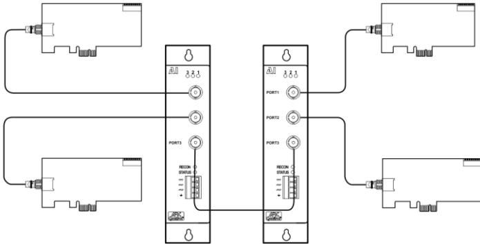
Figure 3 — Point-to-point connections are required between -CXB NIMs and hubs
