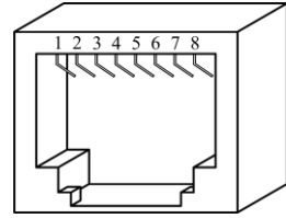
Figure 5 — Modular Jack Numbering Orientation
