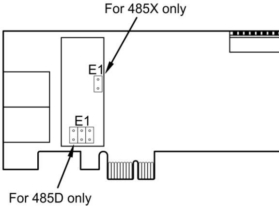
Figure 7 — Jumper settings for EIA-485 models.
