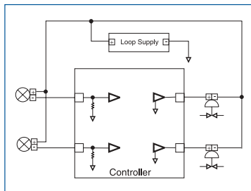
Figure 1. Example of a centralized control system with transmitters on the left and actuators on the right. All input/output devices communicate with a 4-20 mA current loop powered by a single loop supply which is typically 24 VDC.
